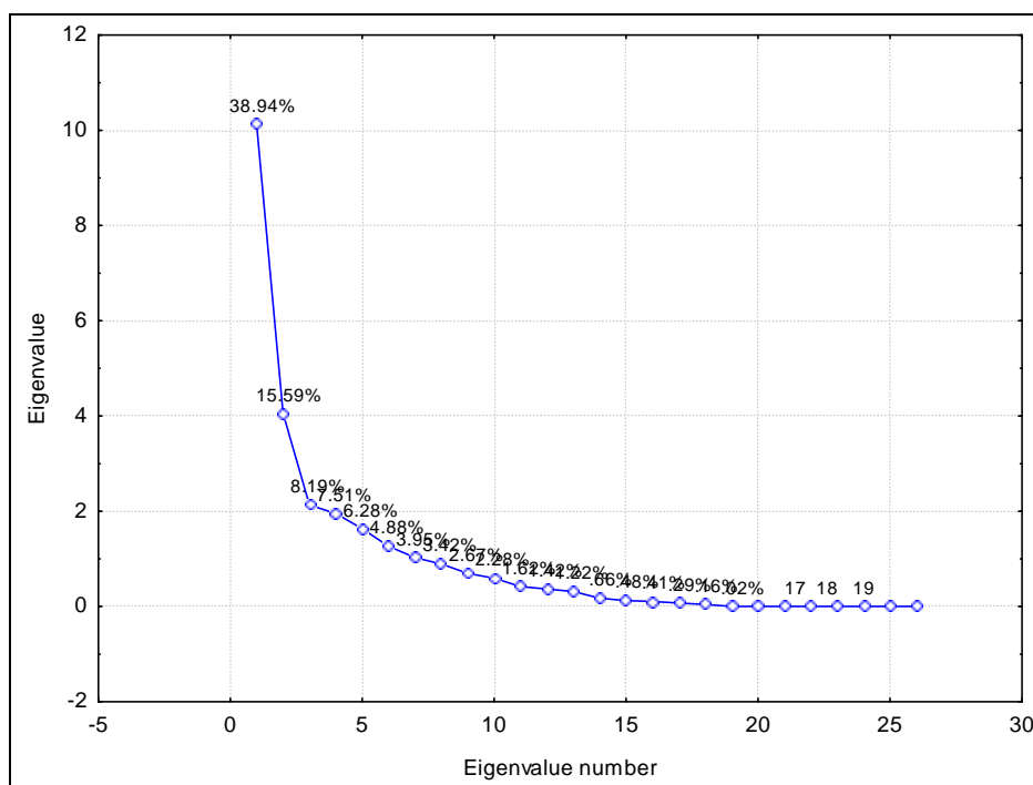
Figure 4.1 Graph showing how much of the total variation in the data set that is explained by each principal component. Eigenvalue number is equal to the principal component number.
