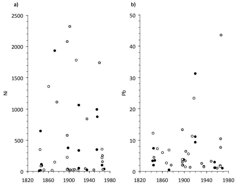
Figure 6. Concentrations ( \mu\text{g/g} ) of a) Ni and b) Pb (the individual seal, yr 1848, with a concentration of 266 \mu\text{g/g} is excluded) in seal bones from Harbor seal (●), Grey seal (○) and Ringed seal over time.
