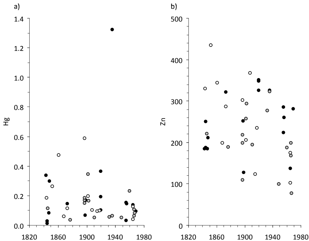
Figure 1. Concentrations ( \mu\text{g/g} ) of a) Hg and b) Zn in individual seal bones from Harbor seal (●), Grey seal (●) and Ringed seal (○, p=0.007 , R^2=0.69 ) over time.
